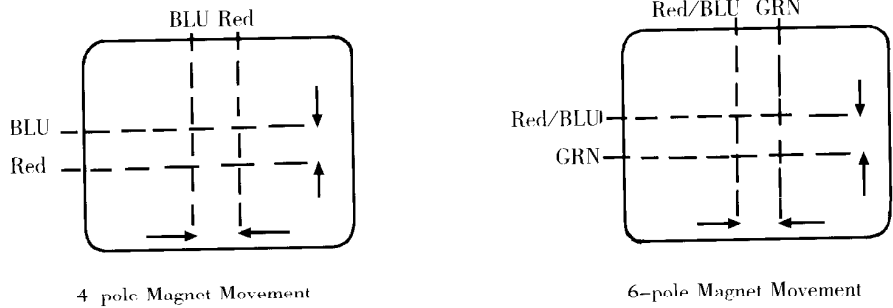
Center Convergence by Convergence Magnets
